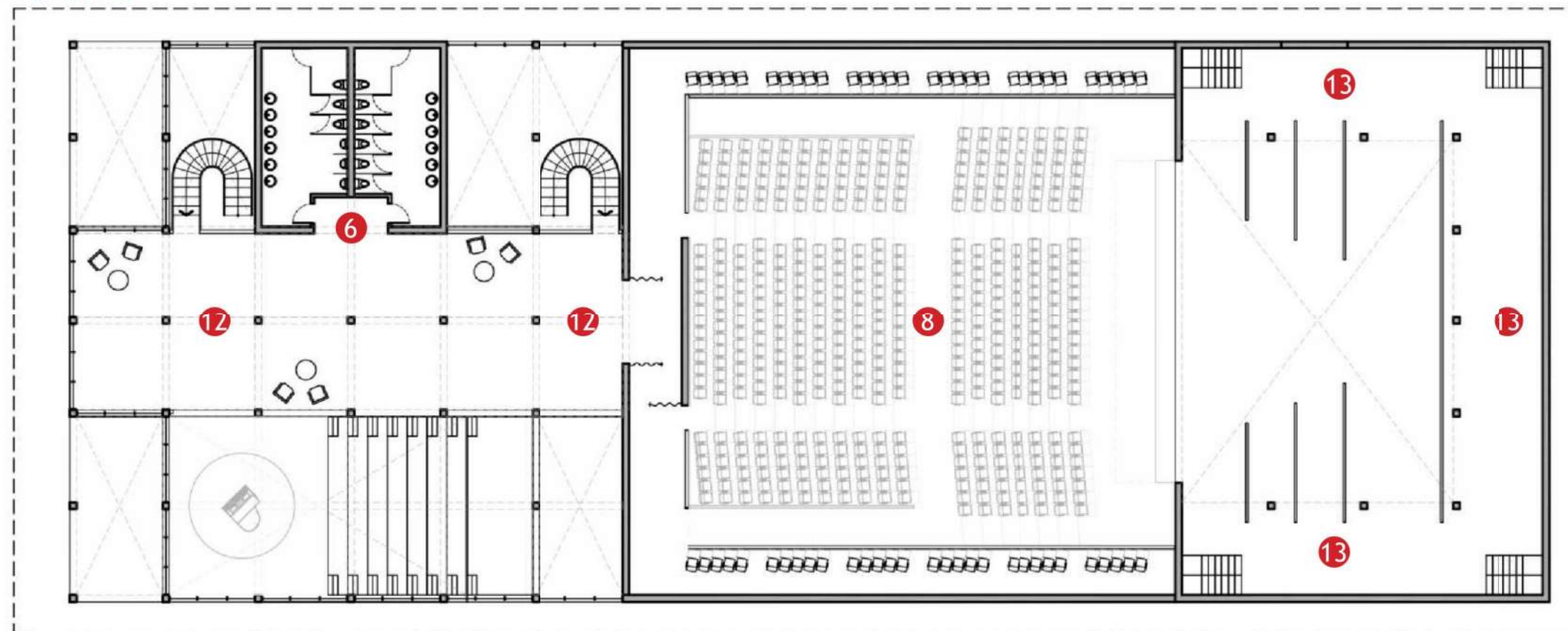
Mezannine
